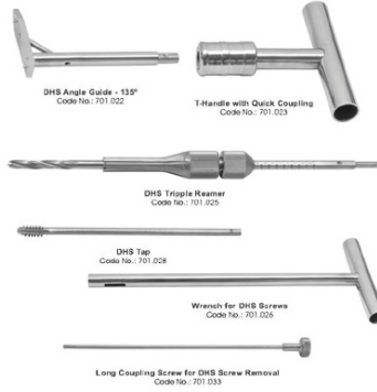
Instruments for DHS - DCS Plates RI-93-1422
