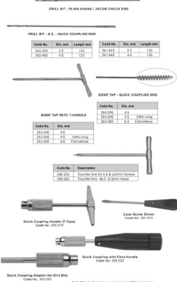
Instruments for Large Fragments RI-93-1434 &nbsp; Instruments for Large Fragments
