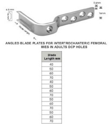
Angled Blade Plates RI-93-1004
