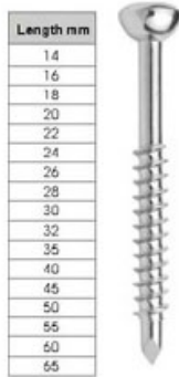
3.5MM MALLEOLAR SCREW
