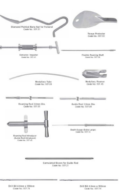
Instruments for RECON Nails RI-93-1447 & Instruments for RECON Nails
