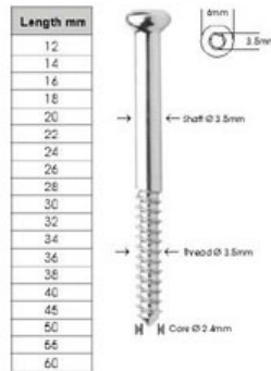
3.5MM SHAFT SCREW FOR LC-DCP
