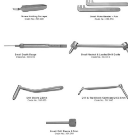
Instruments for Small Fragments RI-93-1451 &nbsp;&nbsp;&nbsp;Instruments for Small Fragments
