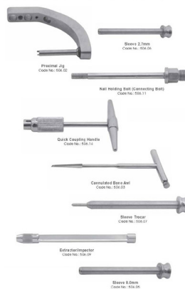
Instruments for Humerus Nails RI-93-1425
