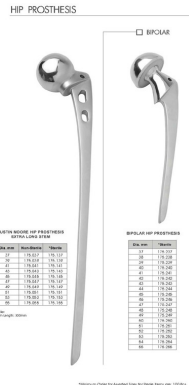
Bipolar Hip Prosthesis - Sterile RI-93-1304 &nbsp;&nbsp;&nbsp;Bipolar Hip Prosthesis - Sterile
