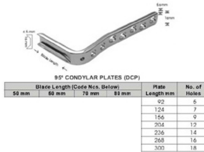
Angled Blade Plates RI-93-1002
