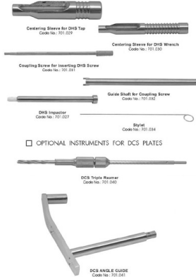
Instruments for DHS - DCS Plates RI-93-1424
