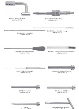
Instruments for Universal Tibia & Femoral Nails RI-93-1454 &nbsp;&nbsp;&nbsp;Instruments for Universal Tibia & Femoral Nails
